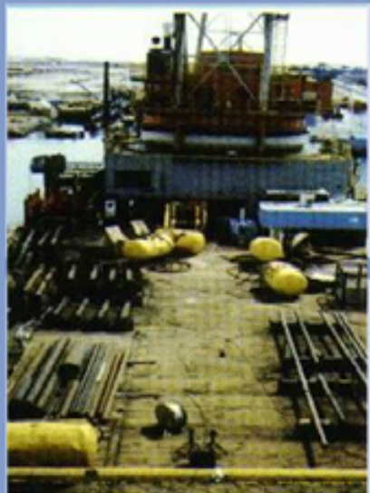
SPM parts on barge deck
